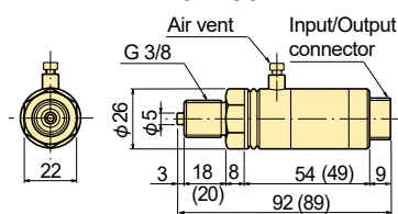
PW-10 ~ 50MPa
