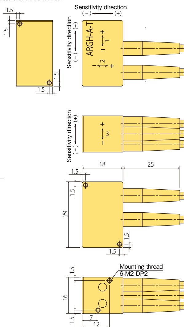
Acceleration transducer
