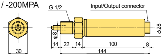
PWH-150 / -200MPa
