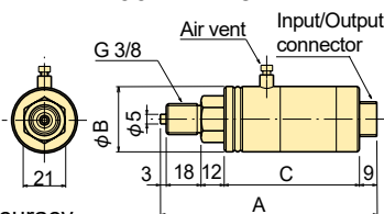
PW-100KPA ~ 5MPa
