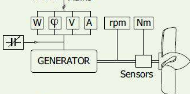
Block diagram
